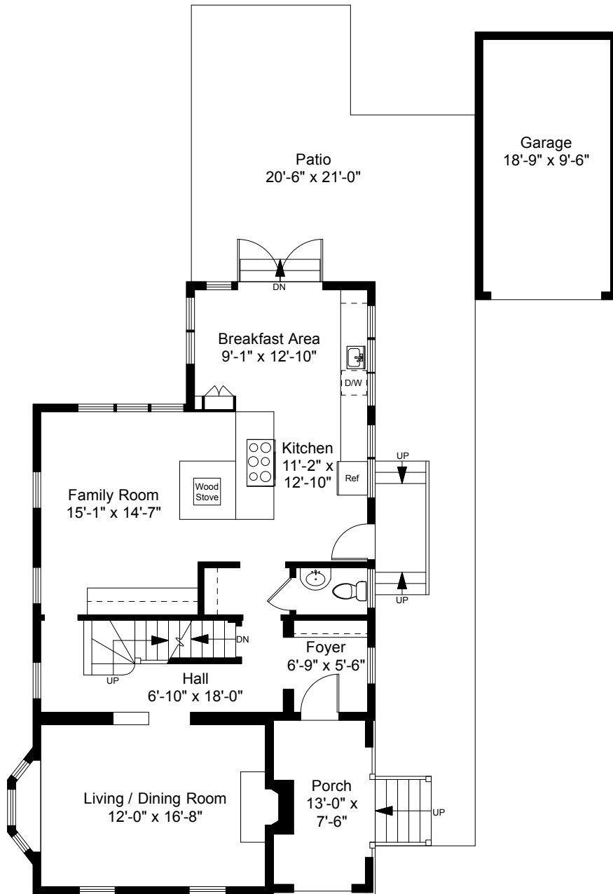
First Floor Plan Ceiling Height = 8'-10"
