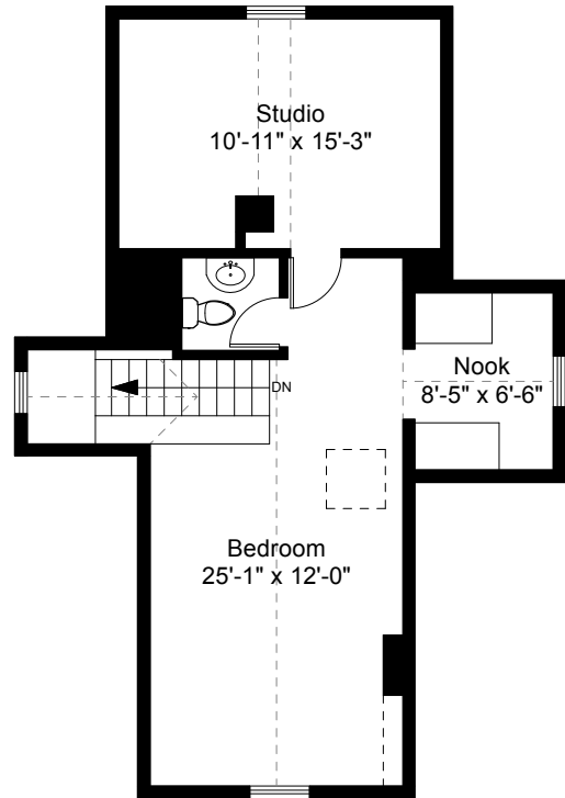
Third Floor Plan Ceiling Height = 8'-9" (At Peak)
