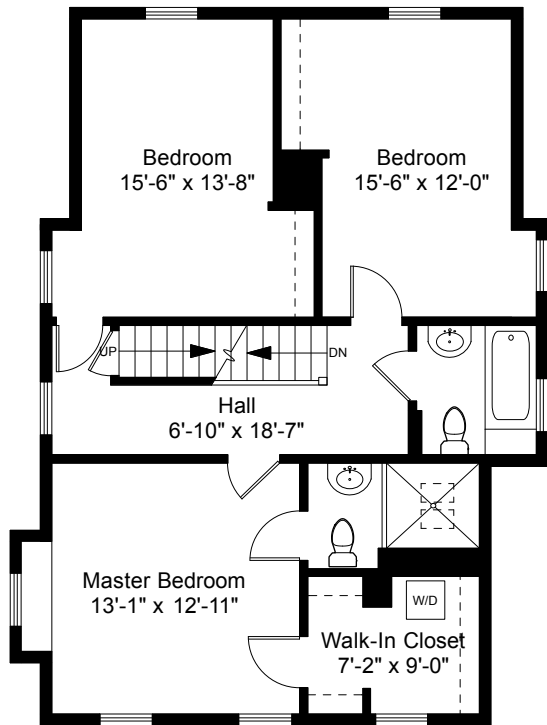
Second Floor Plan Ceiling Height = 8'-10"
